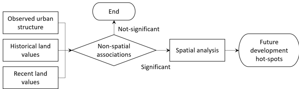
Figure 1: Model's logic
